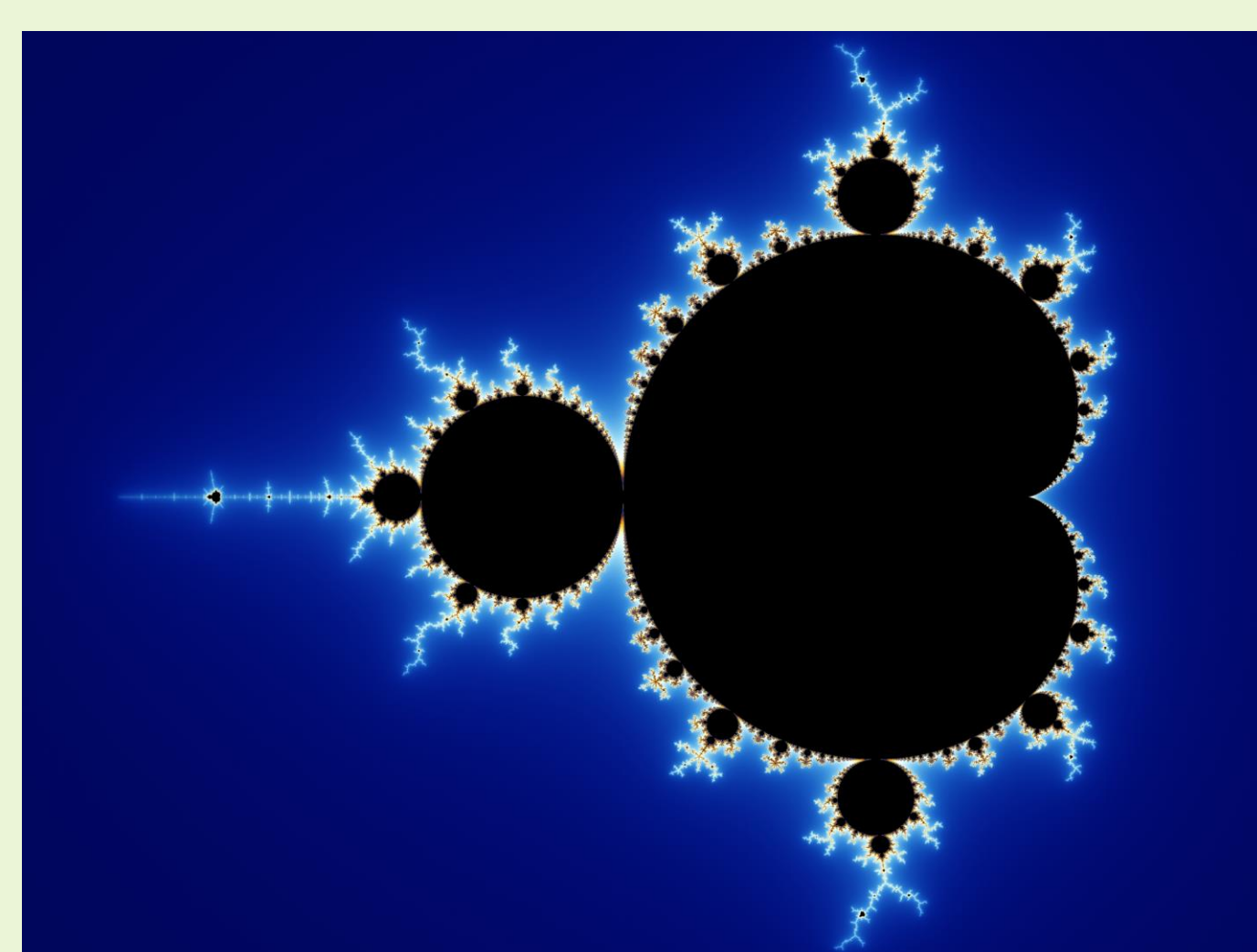
Mandelbrot set
